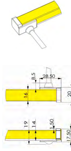
Side Feeder
