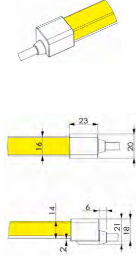
End Feeder
